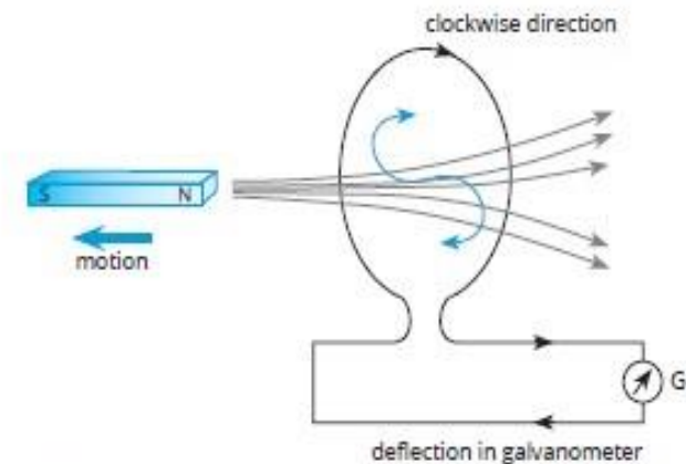
b. N-pole of the magnet moves away from the coil
