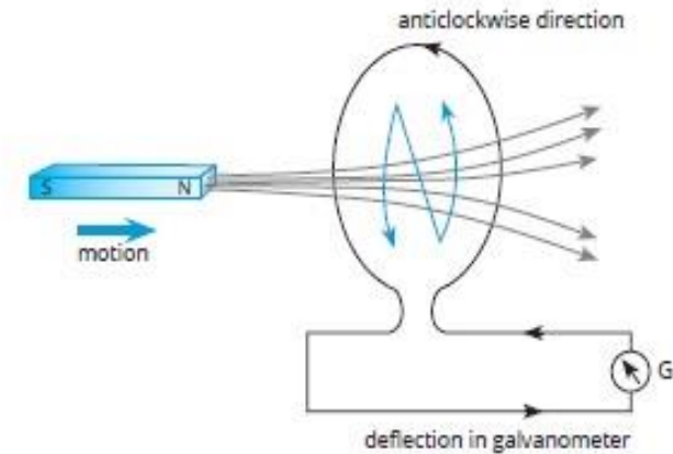
a. N-pole of the magnet moves towards the coil
