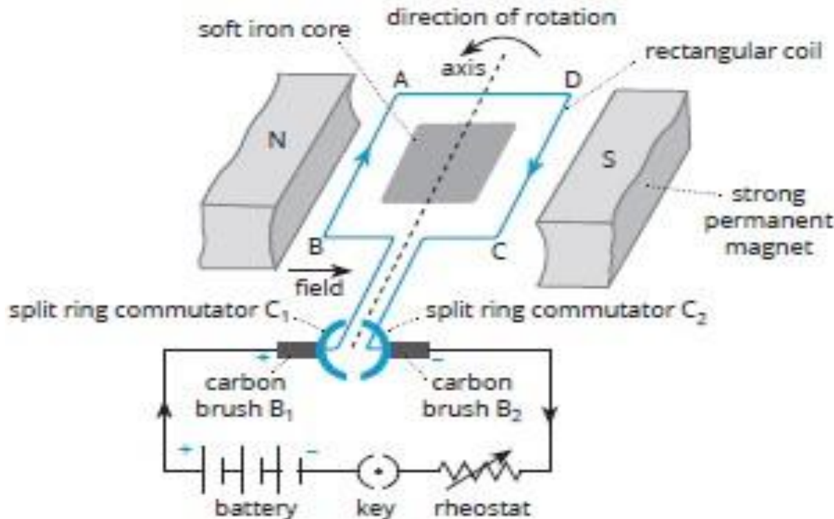
Parts of a DC motor
