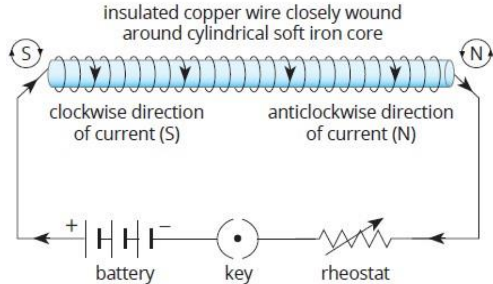
A solenoid
