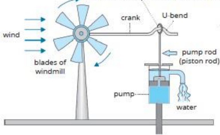
a. Windmill connected to water-lifting pump
