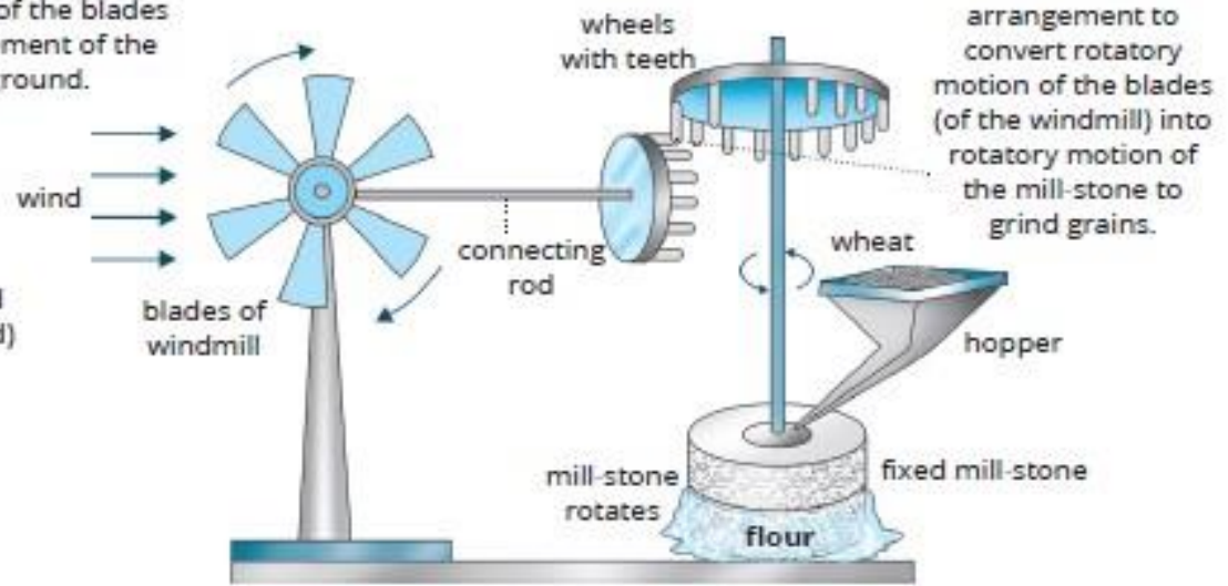
b. Windmill connected to a flour mill
